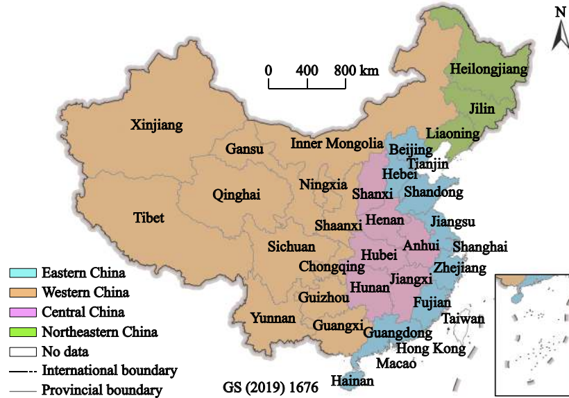
Fig. 1 Administrative division of China. The data do not include Hong Kong, Macao and Taiwan of China
