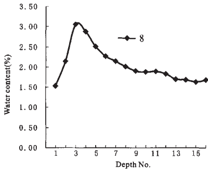
Fig. 4 The third type of the vertical changes of water content in soil in desert (depth unit is 20cm)
