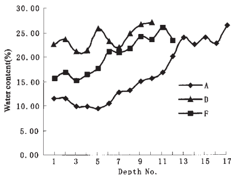
Fig. 6 Vertical changes of water content in oasis (depth unit is 20cm)
