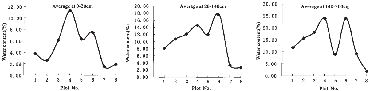
Fig. 5 Horizontal changes of water content from south to north in desert
