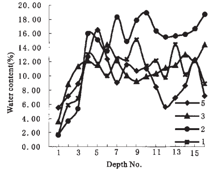
Fig. 2 The first type of the vertical changes of water content in soil in desert(depth unit is 20cm)
