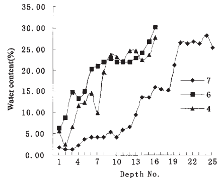
Fig. 3 The second type of the vertical changes of water content in soil in desert(depth unit is 20cm)
