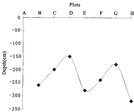
Fig. 1 Changes of ground water table in oasis
